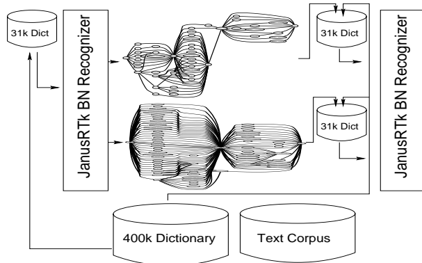
Figure 1: Lexical Adaptation based on Lattices. Two-pass recognition and vocabulary adaptation.
